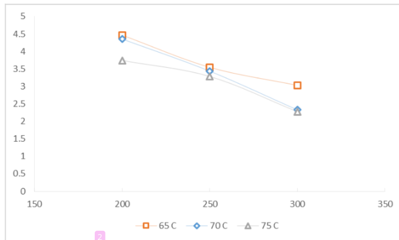
Figure 2. Effect of Alcohol Volume and Temperature on Viscosity
