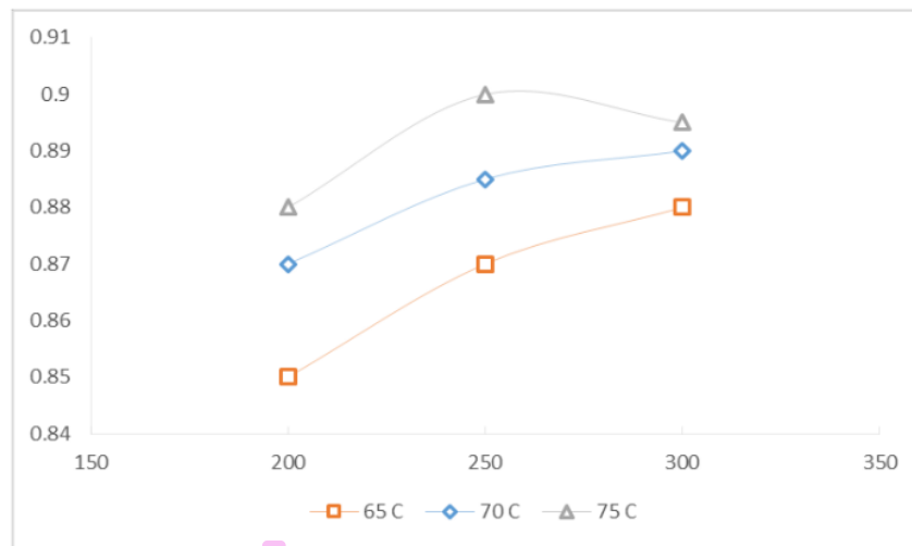
Figure 1. Effect of Alcohol Volume and Temperature on Density
